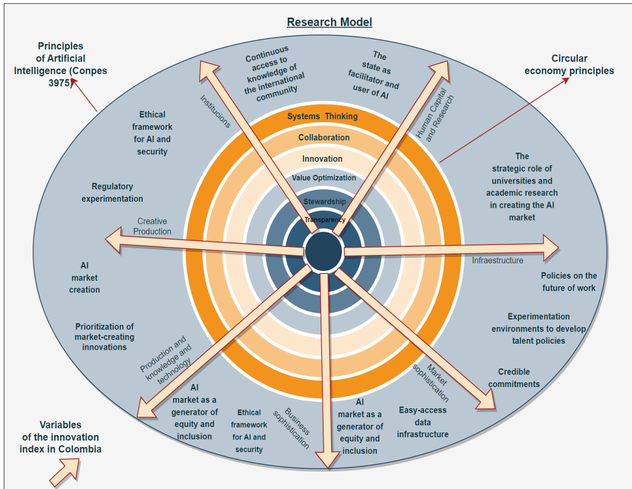
Figure 1. Research variable relationship model.
