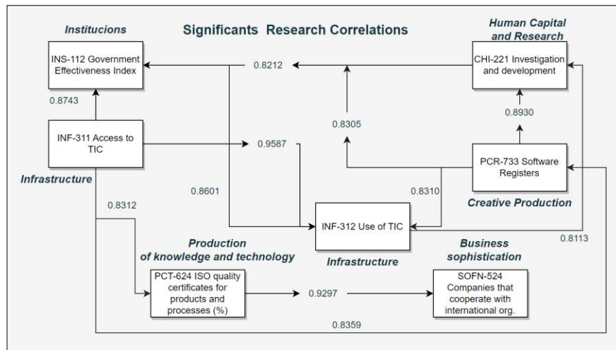
Figure 2. Correlation diagram of research variables
